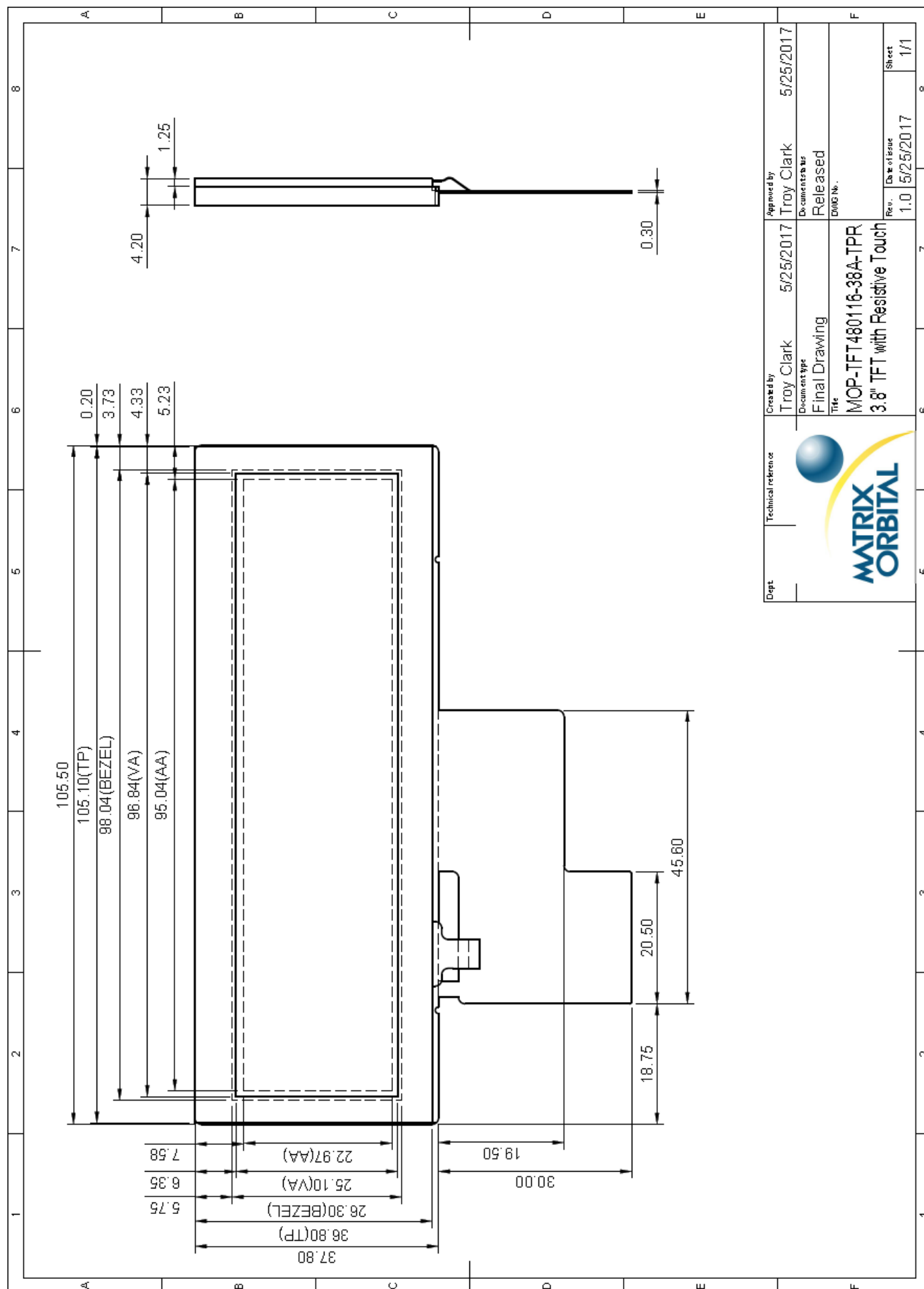
Figure 1: MOP-TFT480116-38A-BLH-TPR Drawing
